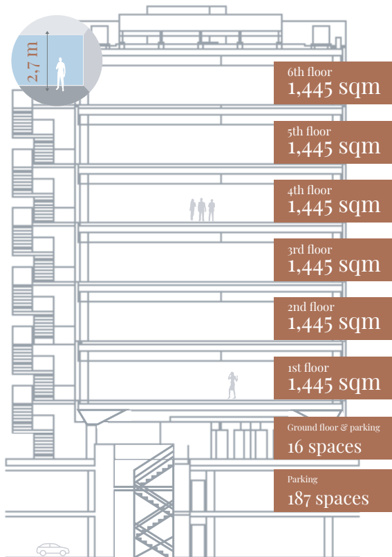
Class A building designed by Valode & Pistre.
