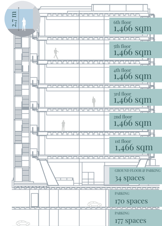
2 Class A twin buildings designed by Carlos Lamela.
