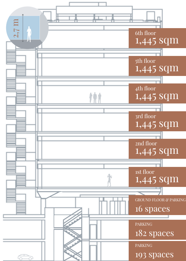
2 Class A twin buildings designed by Valode & Pistre.
